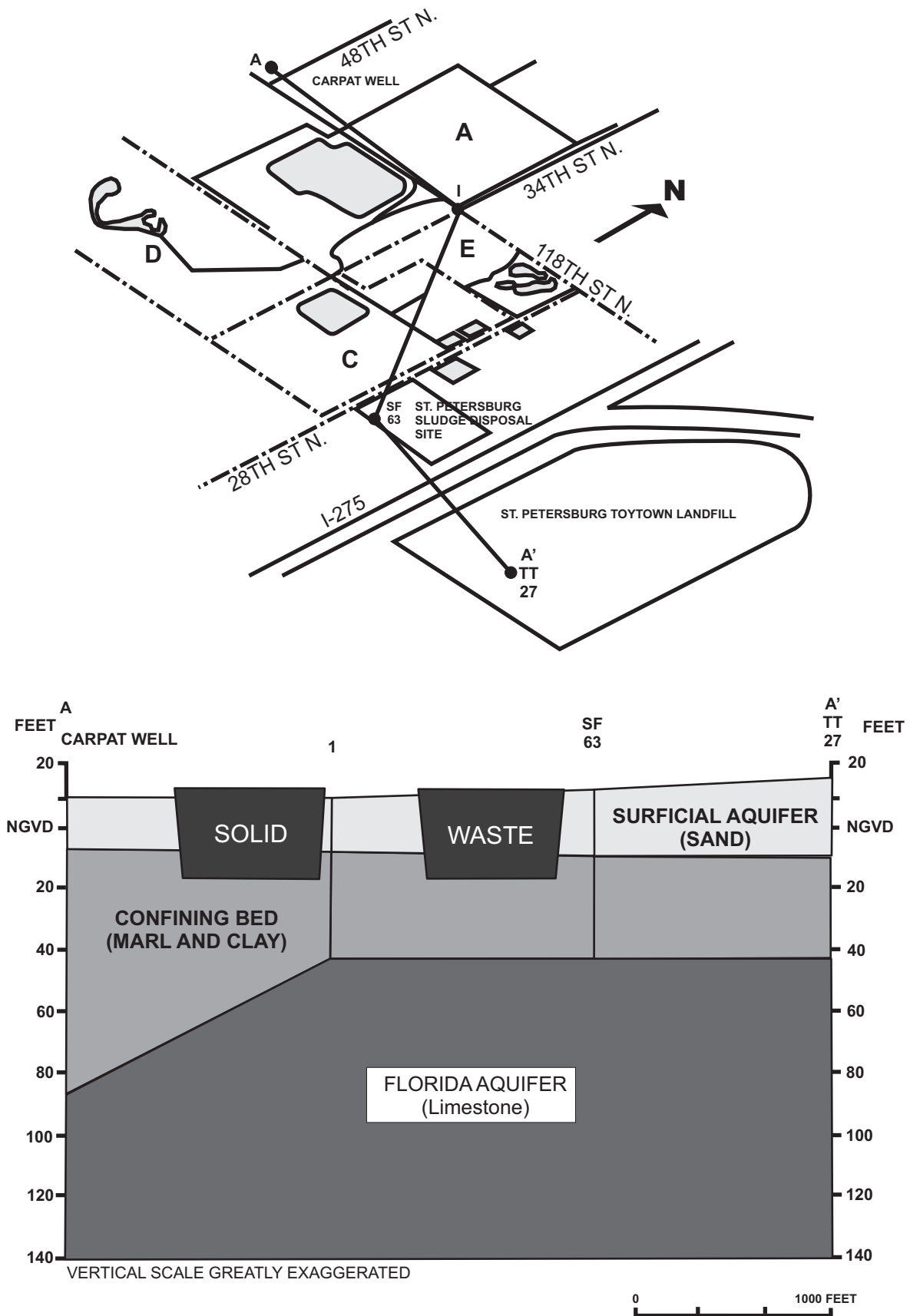
Figure 5 GENERALIZED HYDROGEOLOGIC SECTION AT THE LANDFILL
